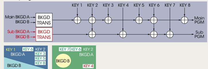
(Fig 1) Multi-program Block Diagram example*
